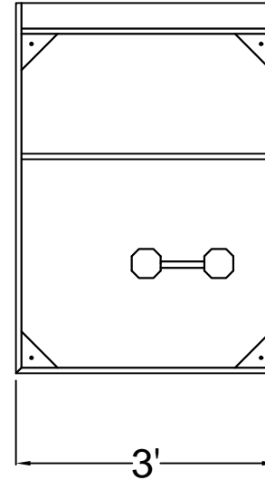
Plan View with 3" insulated rear spacer
