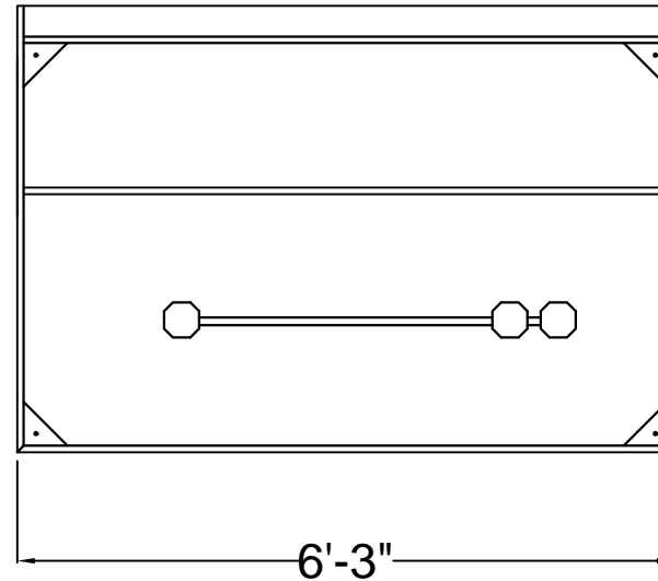
Plan View with 3" insulated rear spacer
