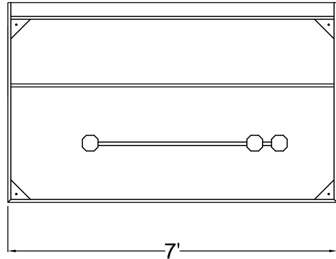
Plan View with 3" insulated rear spacer
