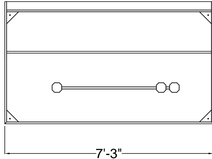
Plan View with 3" insulated rear spacer
