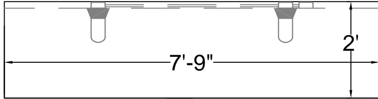
Front View
