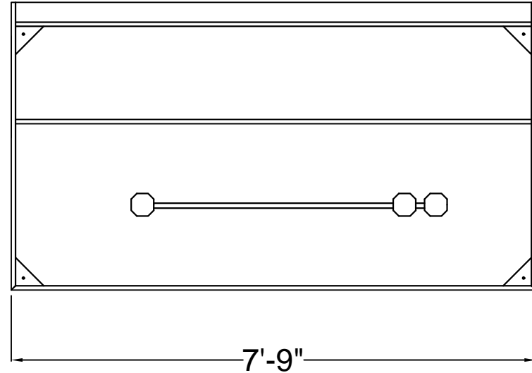
Plan View with 3" insulated rear spacer
