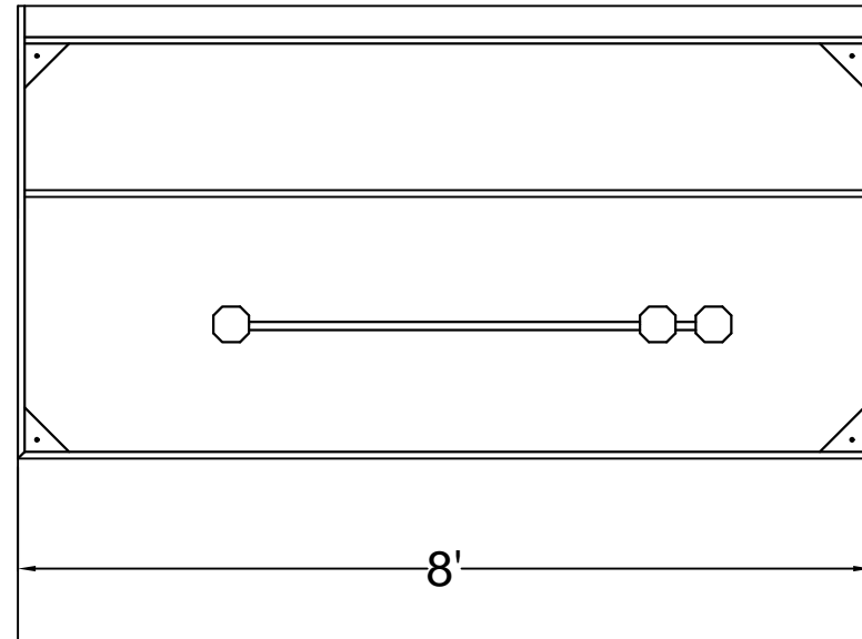
Plan View with 3" insulated rear spacer
