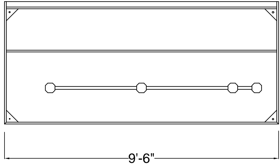
Plan View with 3" insulated rear spacer
