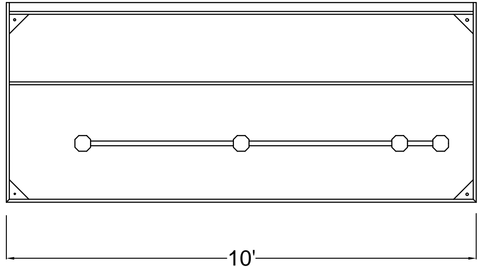
Plan View with 3" insulated rear spacer
