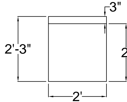
Plan View with 3" insulated rear spacer
