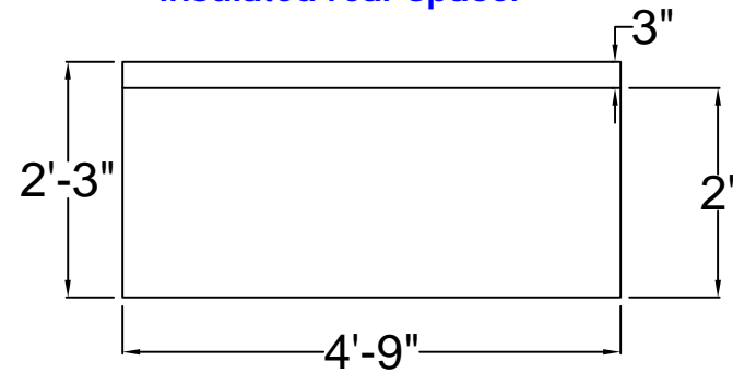
Plan View with 3" insulated rear spacer
