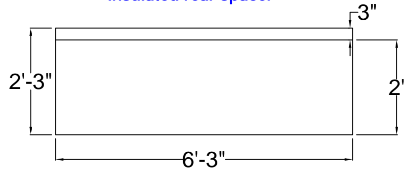
Plan View with 3" insulated rear spacer
