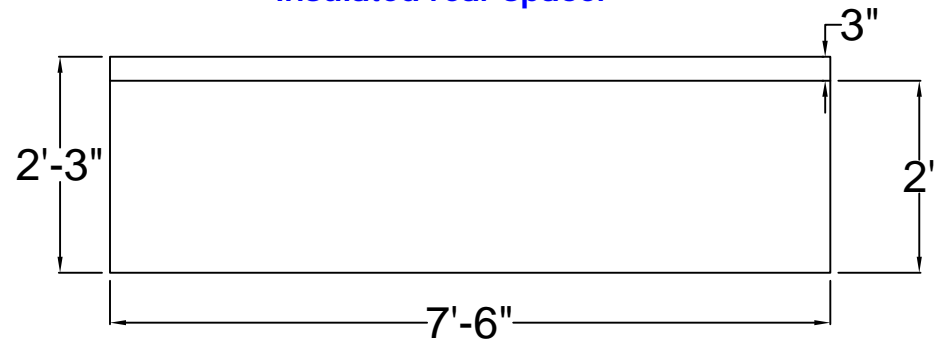
Plan View with 3" insulated rear spacer
