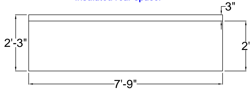
Plan View with 3" insulated rear spacer
